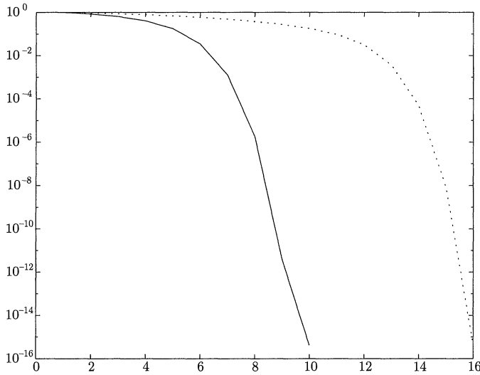
FIGURE 1. Example 1: Quadratic Convergence solid - \delta = 10^{-3} ; dotted - \delta = 10^{-9}
